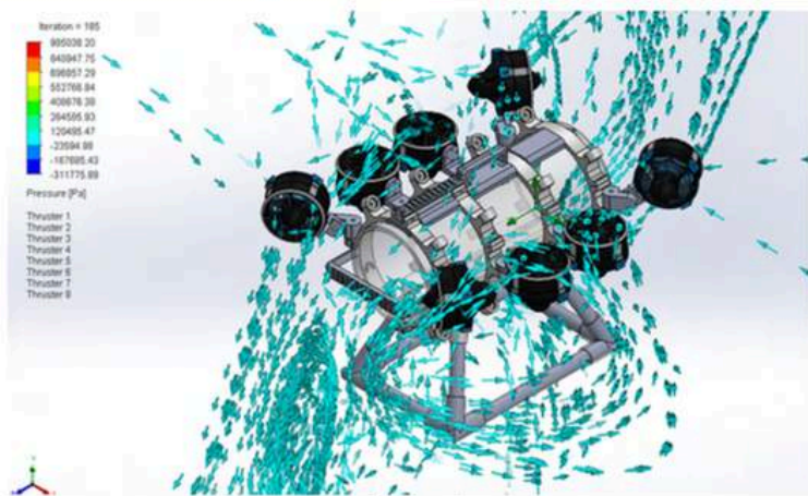
Figure 21, Flow Simulation by Domer Macarine
