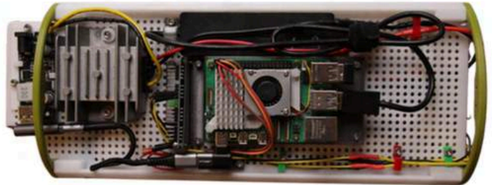
Figure 11, Electrical Layer 1 by Emily Brereton
