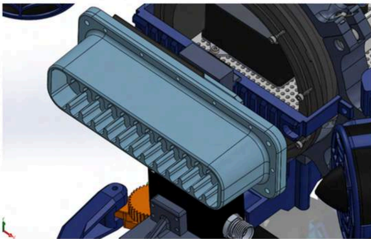
Figure 10, Omniscan Sonar Mounted by Luke Salazar
