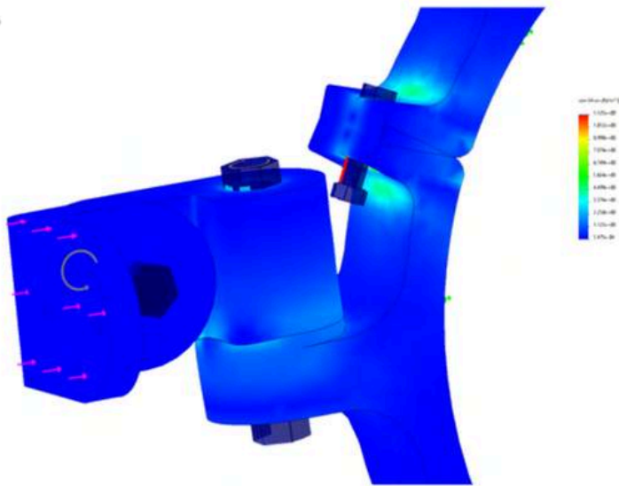
Figure 9 FEA Simulation by Aaron Pruett
