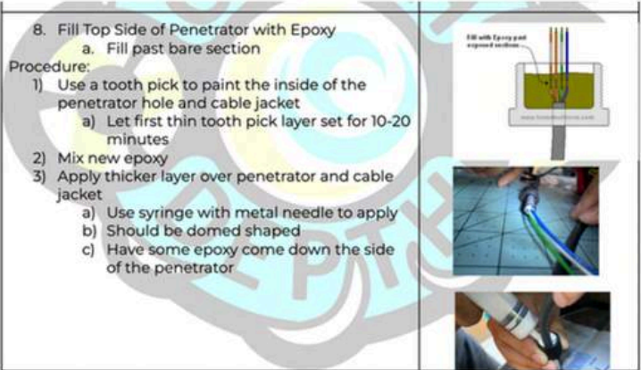
Figure 14, Step 8 CDP_02-Potting Penetrator
